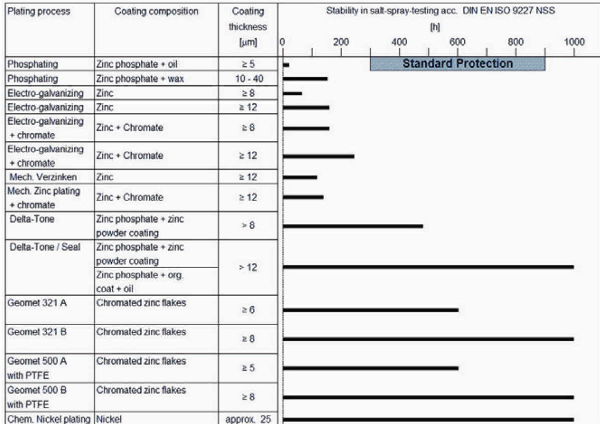
Fig. 3.22: Overview corrosion protection
